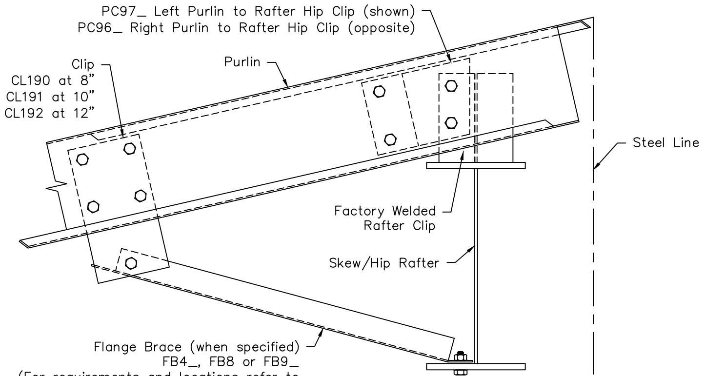
Up Slope View of Purlin to Rafter Connection
